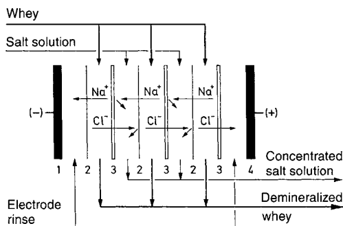
Fig. 10.31. Principle of electrodialysis of whey. 1 cathode, 2 cation membrane, 3 anion membrane, 4 anode
