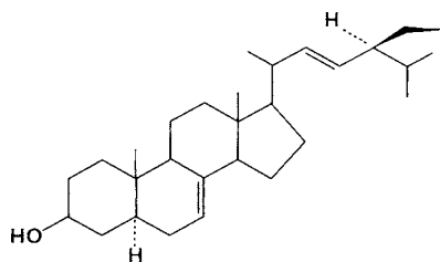
\Delta^7 -Stigmasterol (3.110)
