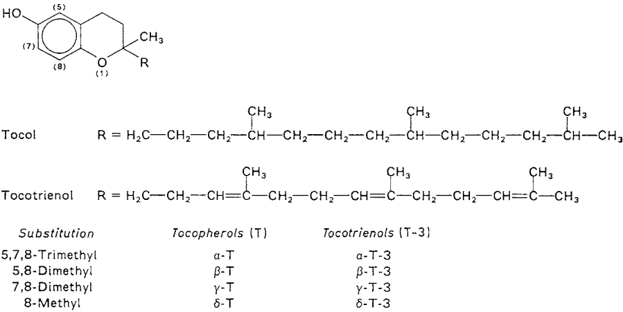
Fig. 3.45. Tocopherols and tocotrienols present in food
