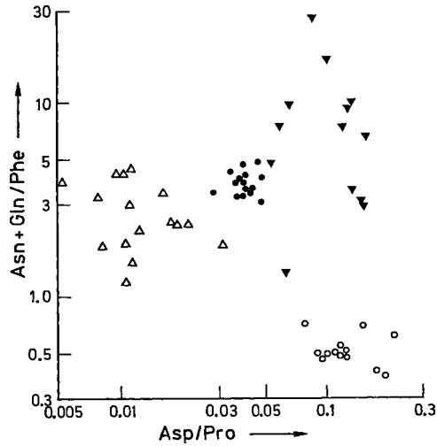
Fig. 19.15. Regional origin of honey as related to its amino acid composition. (according to White, 1978) Honey origin: △ Australia, ● Canada, ▼ United States (clover), ○ Yucatan
