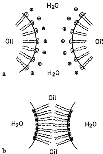
Fig. 8.14. Stabilization of an emulsion. a Activity of an ionic emulsifier in an o/w emulsion. b Activity of a nonpolar emulsifier in w/o emulsion. ○ Polar groups, ~ apolar tails of the emulsifier
