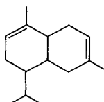
\beta -Cadinene (XLV)
