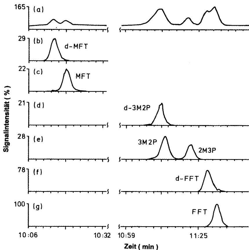
Fig. 5.15. Isotopic dilution analysis of 2-furfurylthiol (FFT), 2-methyl-3-furanthiol (MFT) and 3-mercaptopentan-2-one (3M2P).
