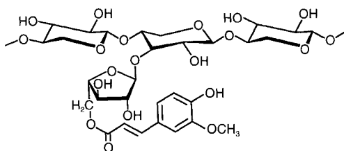
Fig. 15.17. A section of the structure of a water soluble arabinoxylan from wheat. A xylose in the (1 \rightarrow 4)- \beta -xylan section is linked in position 3 with a 5-O-trans-feruloyl- \alpha -L-arabinofuranose
