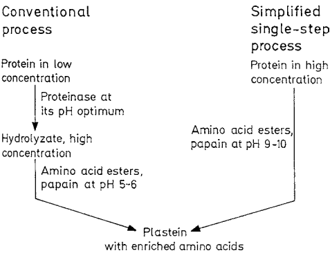
Fig. 1.59. An outline for two- and single-step plastein reactions. (according to Yamashita et al., 1979)
