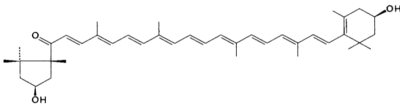
Capsanthin (3,3'-dihydroxy- \beta , \epsilon -carotene-6'-one) (X) (3.129)
