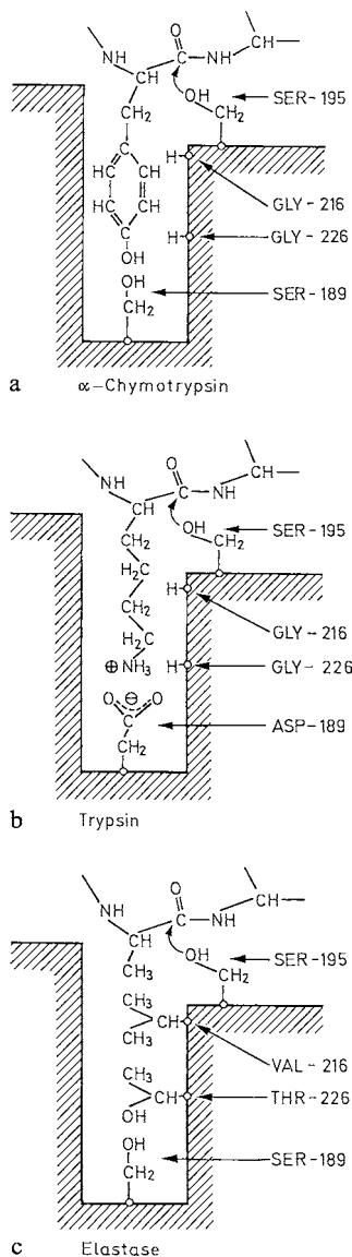
Fig. 2.11. A hypothesis for substrate binding by \alpha -chymotrypsin, trypsin and elastase enzymes (according to Shotton, 1971)
