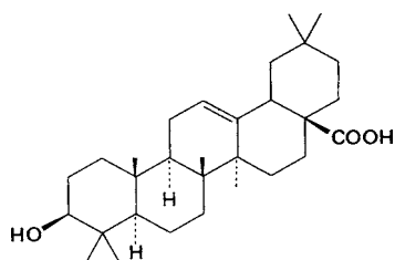
Oleanolic acid
