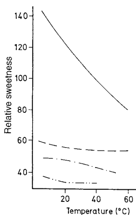
Fig. 4.4. Temperature dependence of the relative sweetness of some sugars (based on saccharose \triangleq 100 at each temperature; — D-fructose, --- D- glucose, -.-.- D-galactose, - - - - maltose) (according to Shallenberger and Birch, 1975 )
