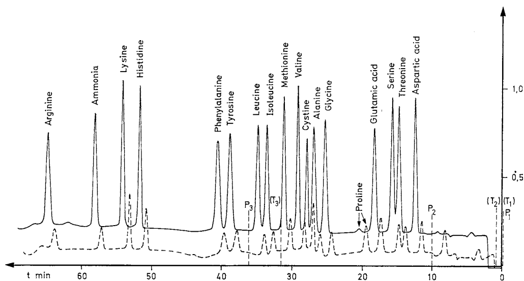
Fig. 1.10. Amino acid chromatogram. Separation of a mixture of amino acids (10 nmol/amino acid) by an amino acid analyzer. Applied is a single ion exchange column: Durrum DC-4A, 295 × 4 mm buffers P 1 /P 2 /P 3 : 0.2 N Na-citrate pH 3.20/0.2 N Na-citrate pH 4.25/1.2 N Na-citrate and NaCl of pH 6.45. Temperatures T 1 /T 2 /T 3 : 48/56/80 °C. Flow rate: 25 ml/h; absorbance reading after color development with ninhydrin at 570/440 nm: —/— — — —
